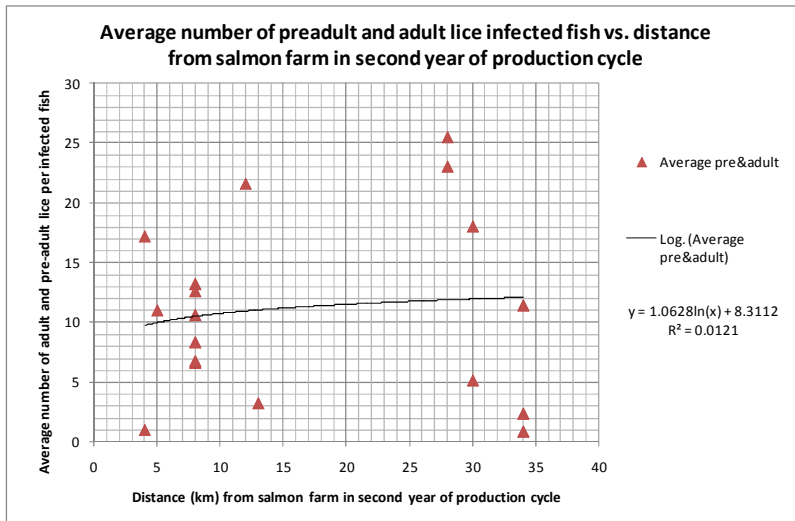
Figure 4.13 Average number of pre-adult and adult lice per infected sea trout in samples vs. distance from salmon farm in second year of the production cycle (excluding Kanaird, 8 May 2008 sample).
