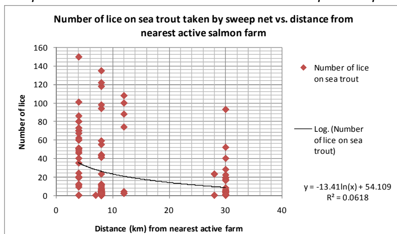
Figure 4.8 Total numbers of lice per sea trout taken in sweep net samples taken in WRFT area in 2008 vs. distance from the nearest active salmon farm. Excludes fish taken in sample on 8 th May 2008; a sea trout with 500 lice taken in the Carron in May 2008. Boor Bay samples have been limited to a random 20 fish per sample.
